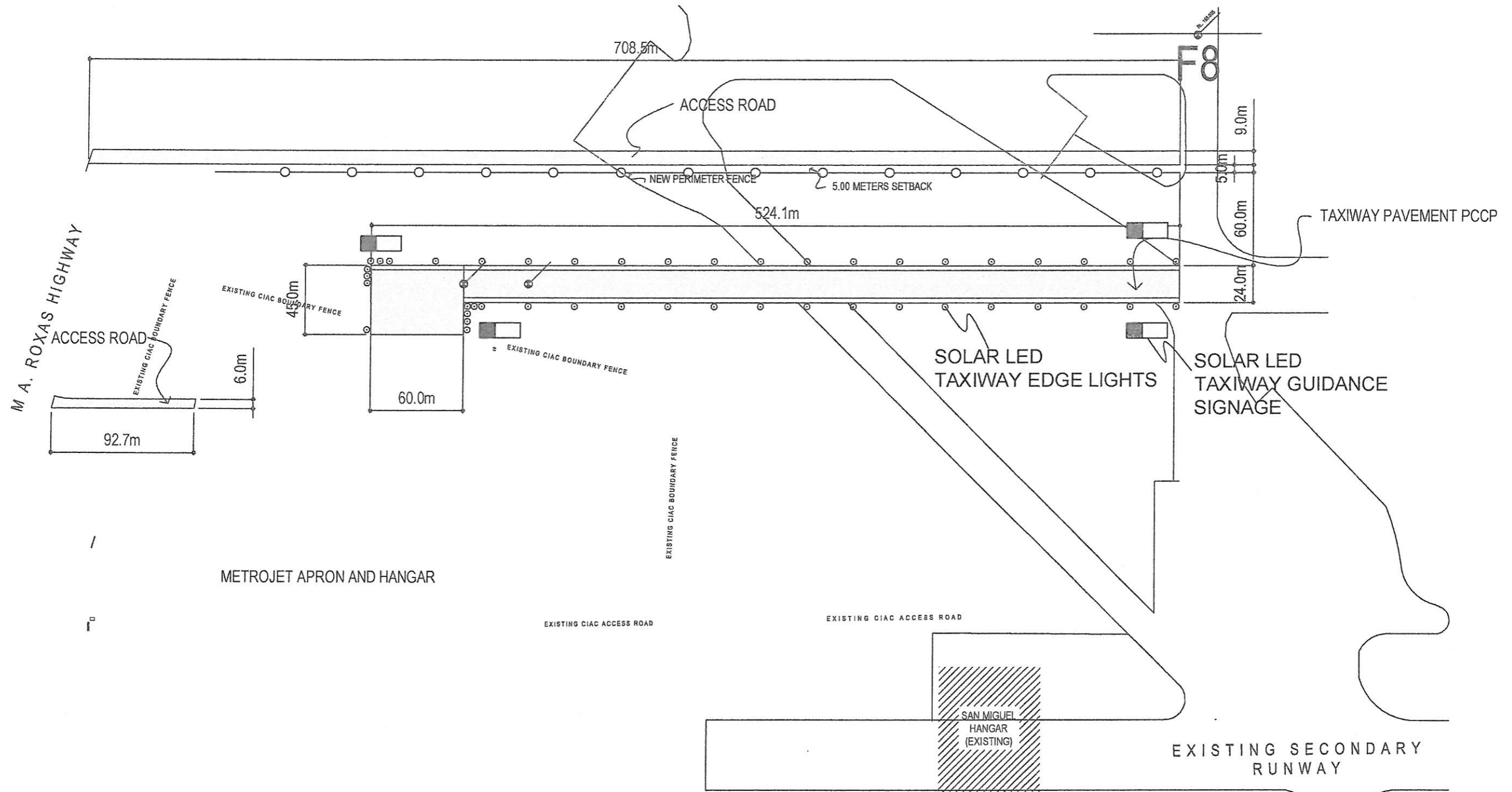
A TAXIWAY LIGHTINGS LAYOUT TP-2 SCALE: 1:1000 MTS.
