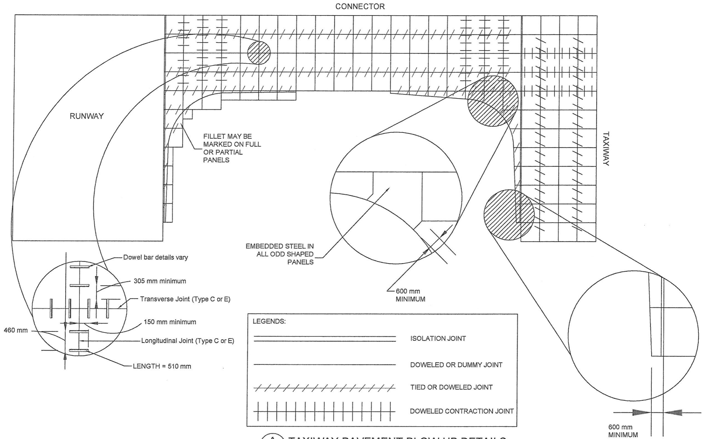
A TAXIWAY PAVEMENT BLOW-UP DETAILS TP-2 SCALE: N.T.S.
