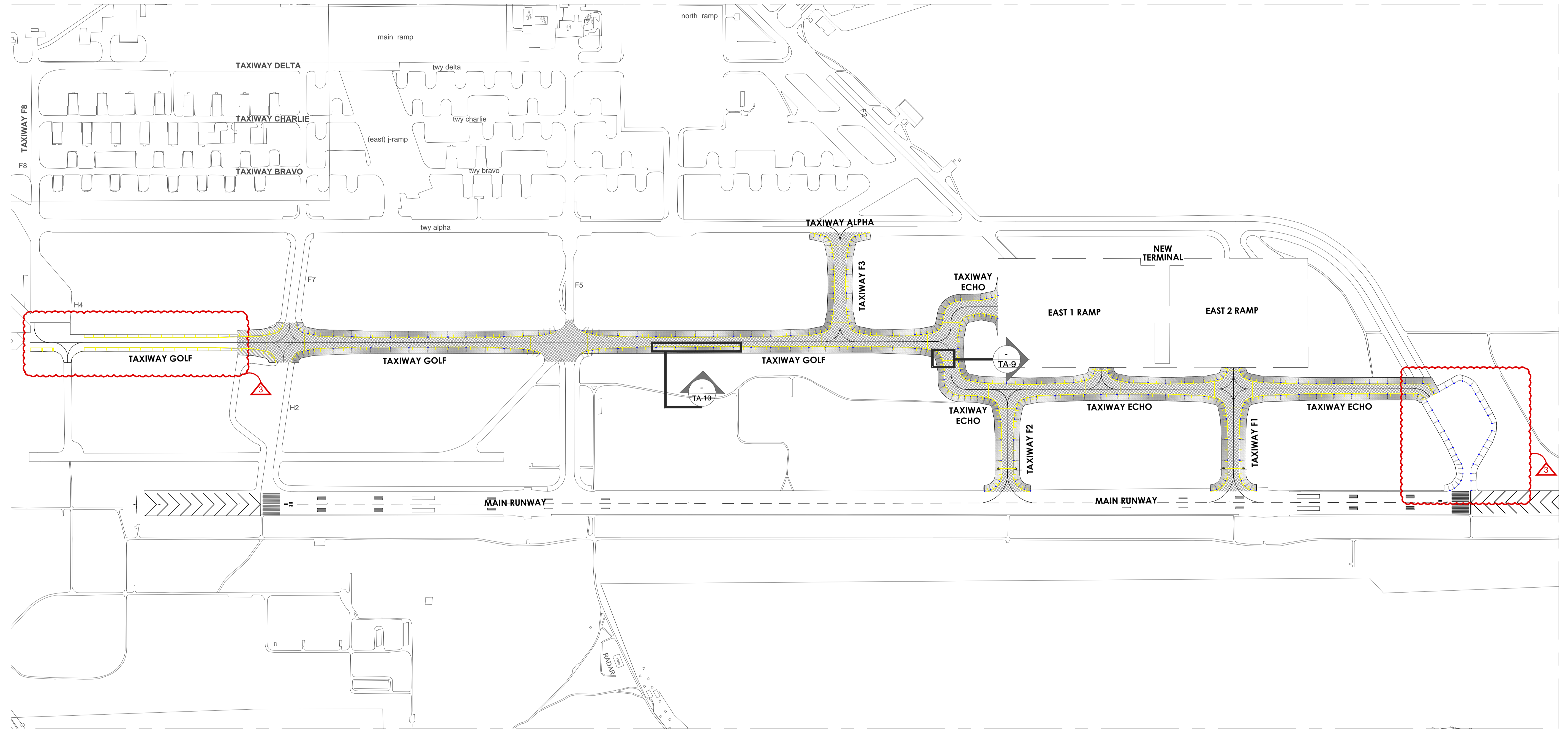
A TAXIWAY EDGE LIGHTING LAYOUT SCALE 1:5500MTS.
