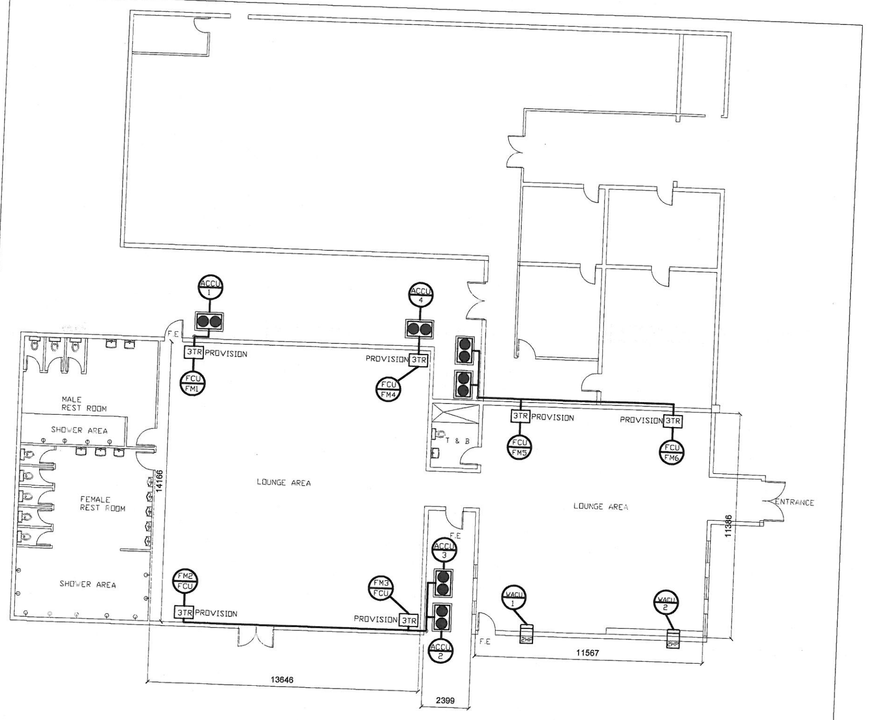
SECURITY LOUNGE PROPOSED MECHANICAL FLOOR PLAN SCALE: 1:100 MTS
