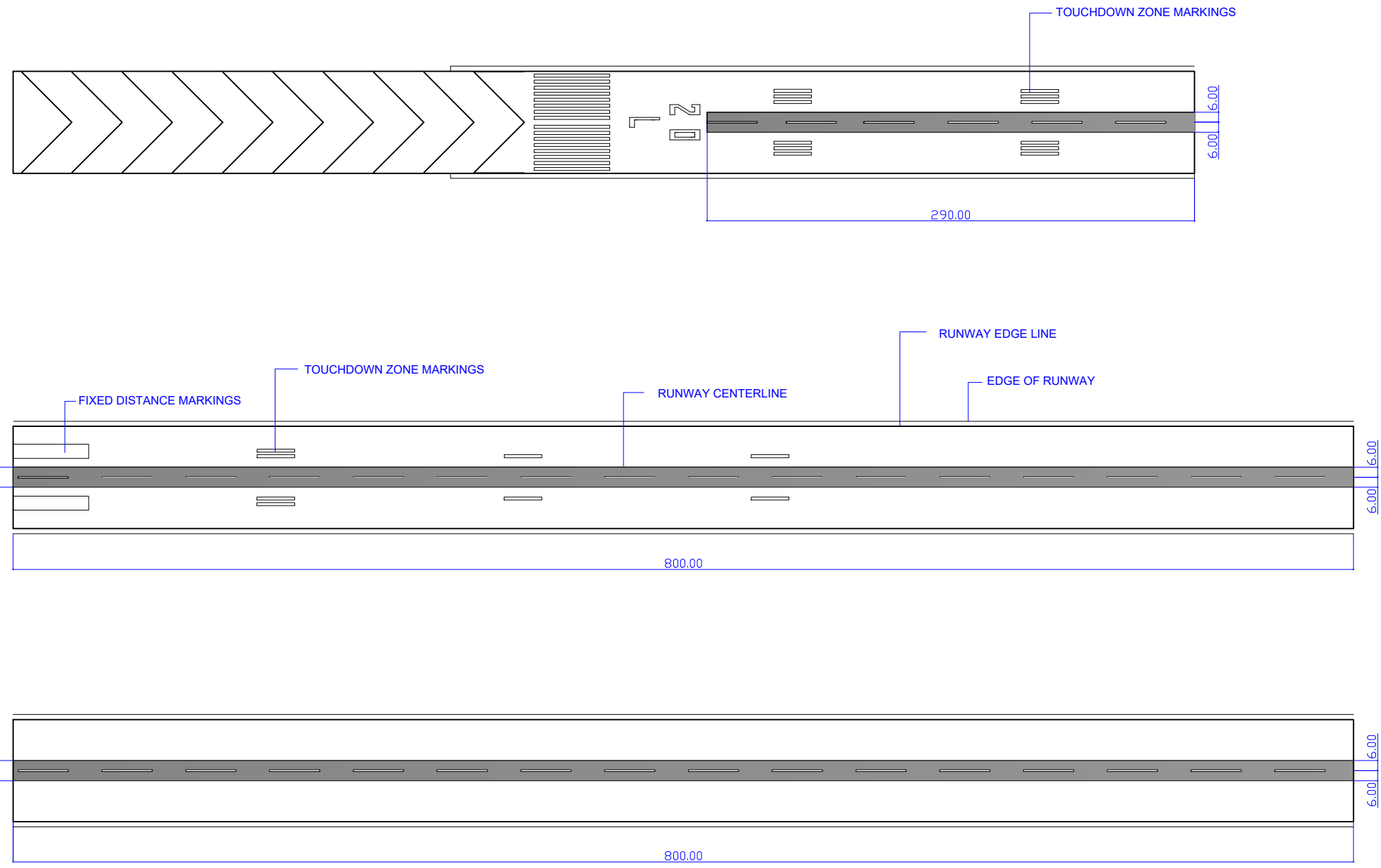
PLAN OF FRICTION TEST RUN AT RUNWAY 20L
